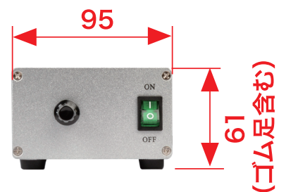
[正面]
