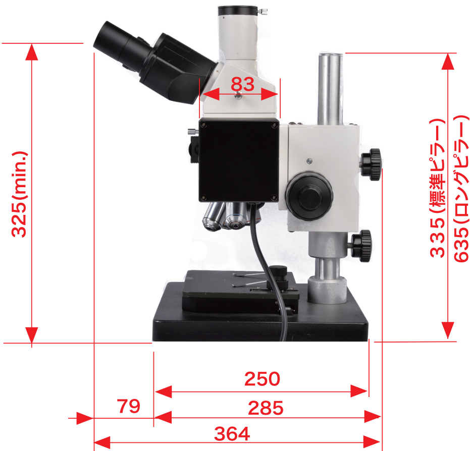
[右側面]
